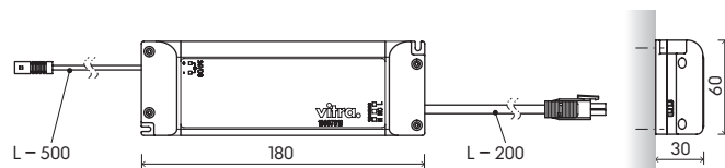
Fig. 11: Converter dimensions
