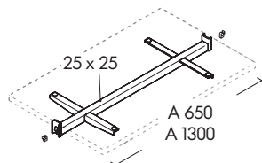
Fig. 5: Back bar for shelf without electrification
