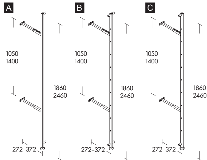
Fig. 3: Wall uprights
